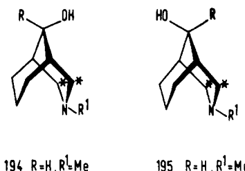
194 R = H, R 1 = Me
