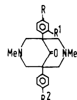
182a R = R 2 = H, R 1 = NO 2 182b R = R 2 = NO 2 , R 1 = H 182c R = R 2 = H, R 1 = Me
